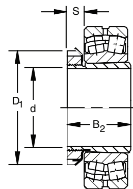
Tapered bore bearing plus SNW.
